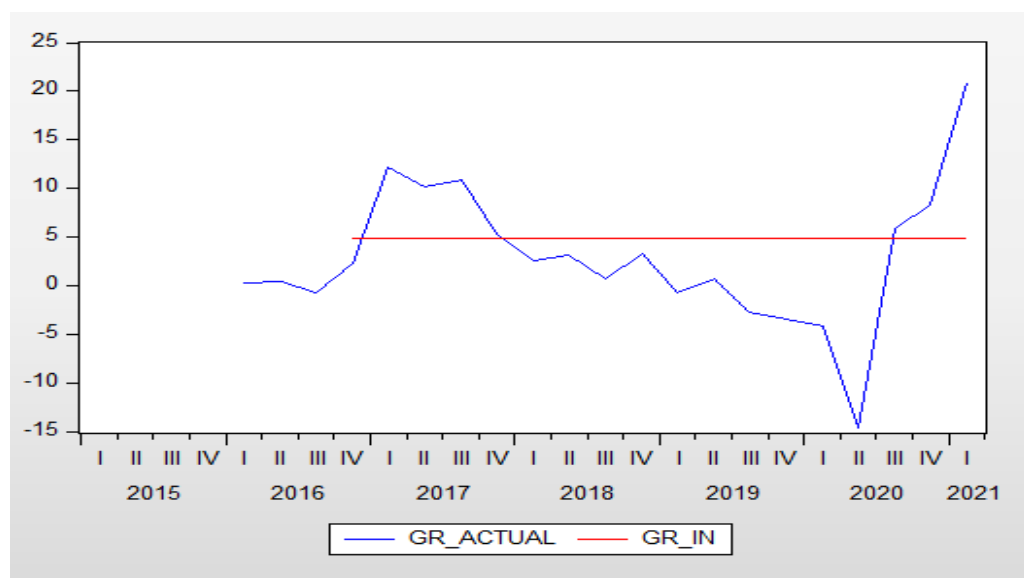
Figure 5.8: The comparison of the actual and in sample forecast growth.
